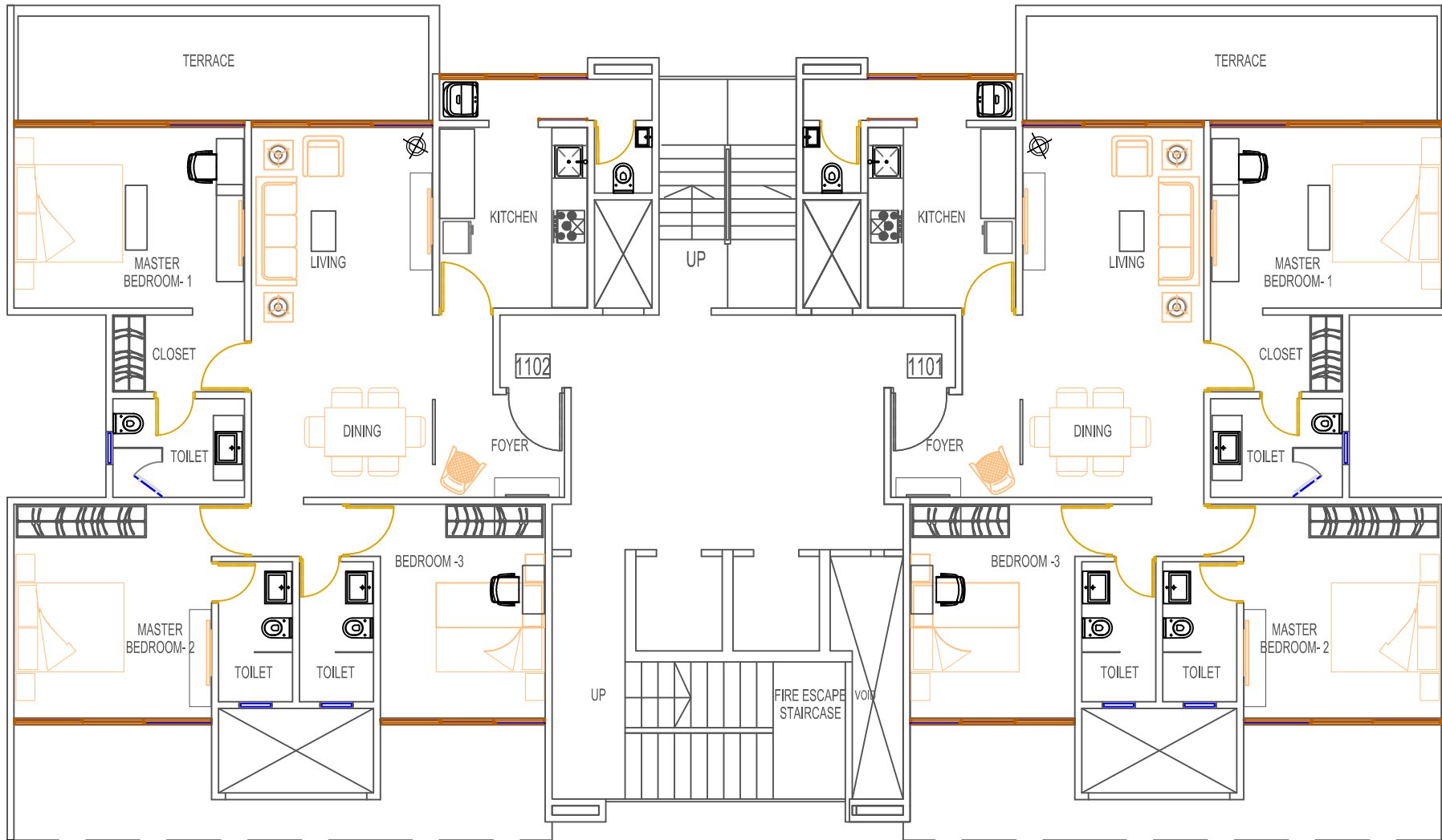
BUILDINGS NO. III & IV ODD-FLOOR PLAN
